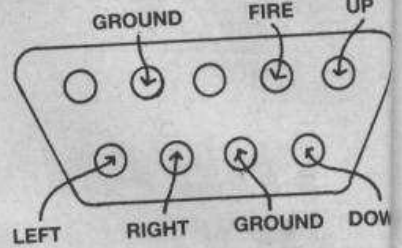
Spectrum Plus Two joystick socket wiring (view of socket 1 or 2)
